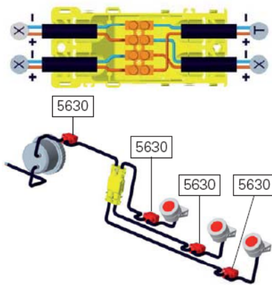
3 LED spotlights serial connected with driver
