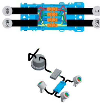
3 LED RGB spotlights (cable with 4conductors) parallel connected to RGB station controller
